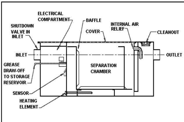
Figure 12: Sensor controlled Grease Recovery Device (GRD)
