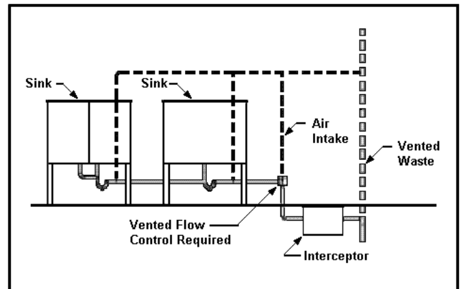
Figure 8: Grease Interceptor serving two individually trapped and vented sinks – flow control air intakes intersects vent.
